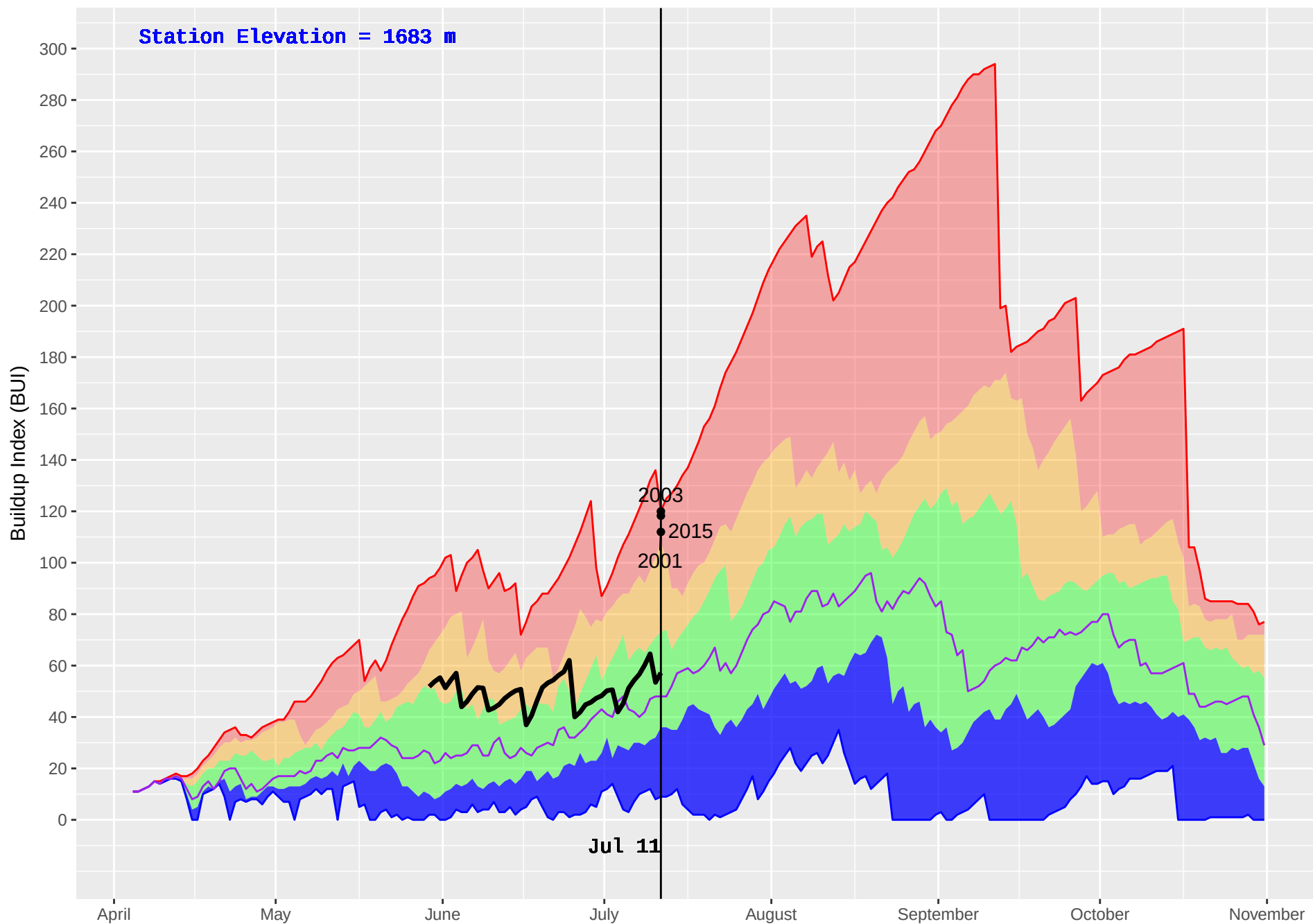
ASHNOLA (331) : Historical (1992–2016) and Current (2018) Noon Buildup Index (BUI)
