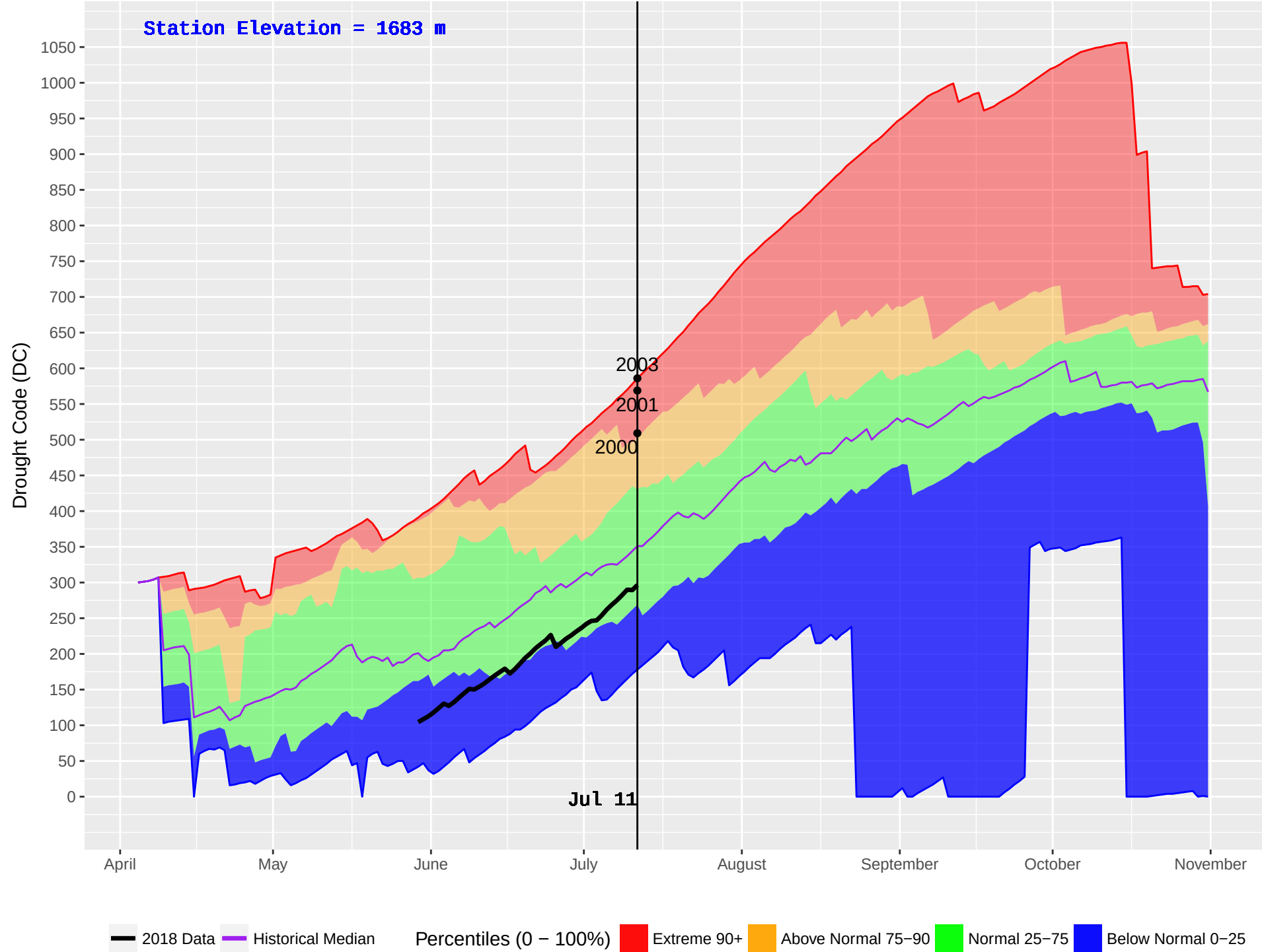
ASHNOLA (331) : Historical (1992–2016) and Current (2018) Noon Drought Code (DC)
